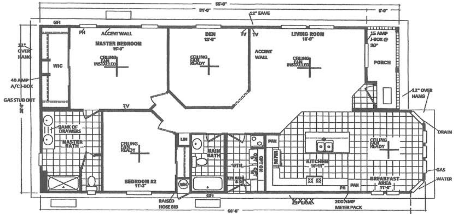
CATALINA MODEL APPROX. 1,541 SQ. FT. INCLUDING PORCH 2 BEDROOM, DEN, 2 BATH
